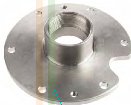
VP2 BYPASS ADAPTER R2" FOR PLUGSY 200-400 (8"-16") 520344
